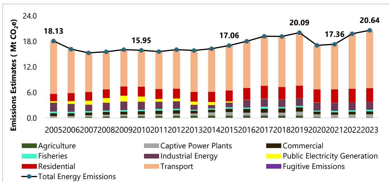
Figure 1: GHG Emissions Estimates of Energy Sector – Kerala (2005 to 2023)
