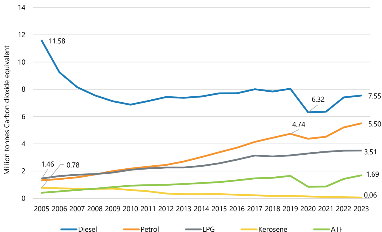
Figure-ER-11: Long-term Emissions Trend – Major Fuel Categories – The figure shows the Long-term trend of liquid/ gaseous fuels that have the highest contribution to the total emission in the Energy Sector. There are combustion emissions from other fuels accounted for in the emission inventory including Naphtha and natural gas which are not represented in the graph. [LPG- Liquefied Petroleum Gas, ATF- Aviation Turbine Fuel]
