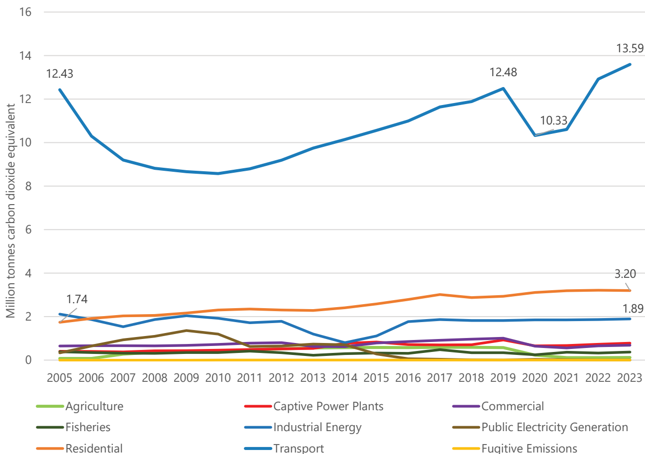
Figure-ER-9: Long-term Emission trend-Energy use categories - Shows the Long-term trend in emissions from the various emission sources in the Energy sector contributing to the overall sector emission. Transport emissions are the cumulated emissions from various sources like road transport, railways, aviation and navigation.
