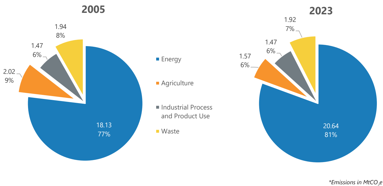
Figure ER-5: Kerala-IPCC Sector based emissions and percentage shares in the Long-term
