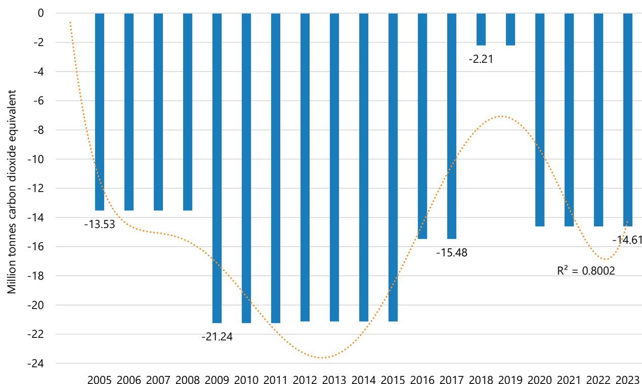
Figure ER-4: Total Removals in the Long term from sink categories in the state. The figure shows the quantity of atmospheric CO 2 sequestered as carbon in vegetation and soils in terrestrial ecosystems. The dotted line shows the best-fit trendline.
