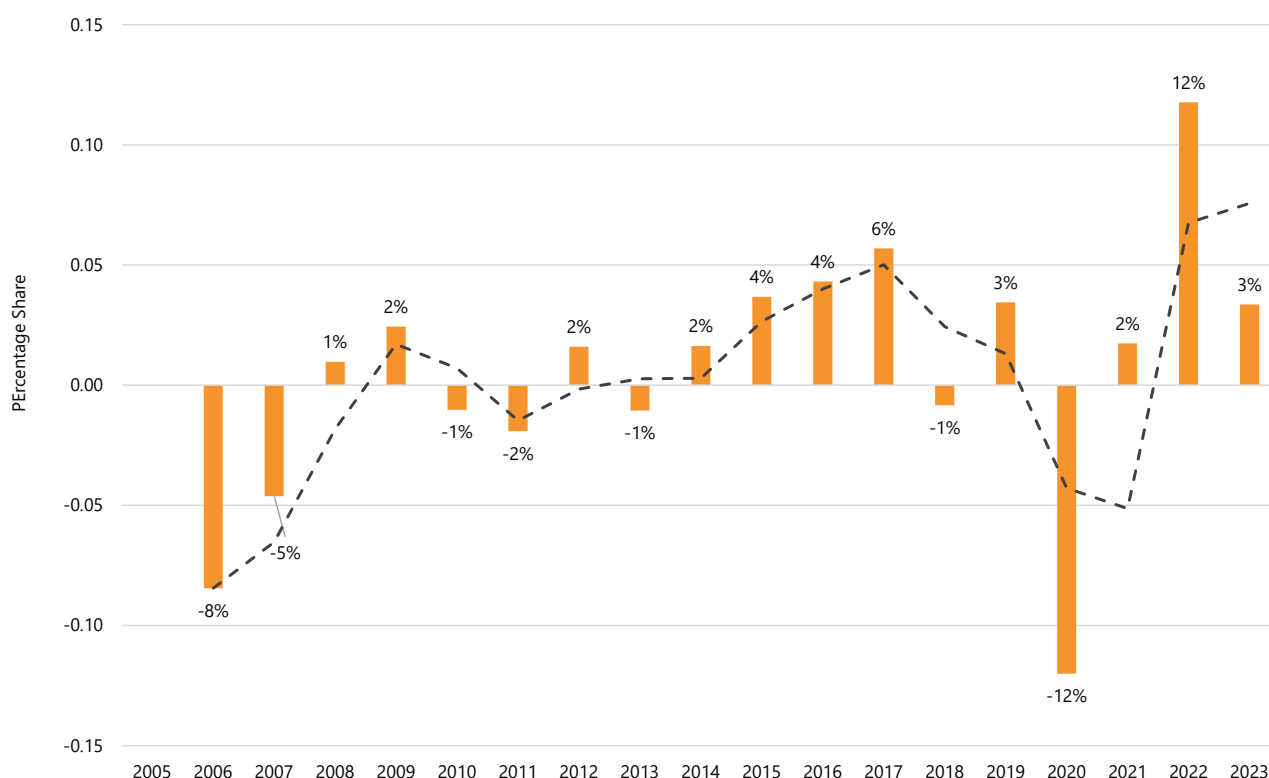
Figure-ER-3: Long-term percentage changes (Year-on-Year) in gross greenhouse gas emissions, Kerala. The dotted line shows the trend in the changes (two-period moving average).
