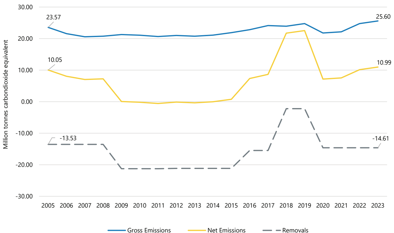
Figure-ER-1: Kerala Long-term Gross & Net Greenhouse Gas Emissions and Removals - Shows the overall trends in Greenhouse Gas emissions from Kerala in the long term (2005-2023). The dotted line shows the total CO 2 removals through carbon sequestration.
