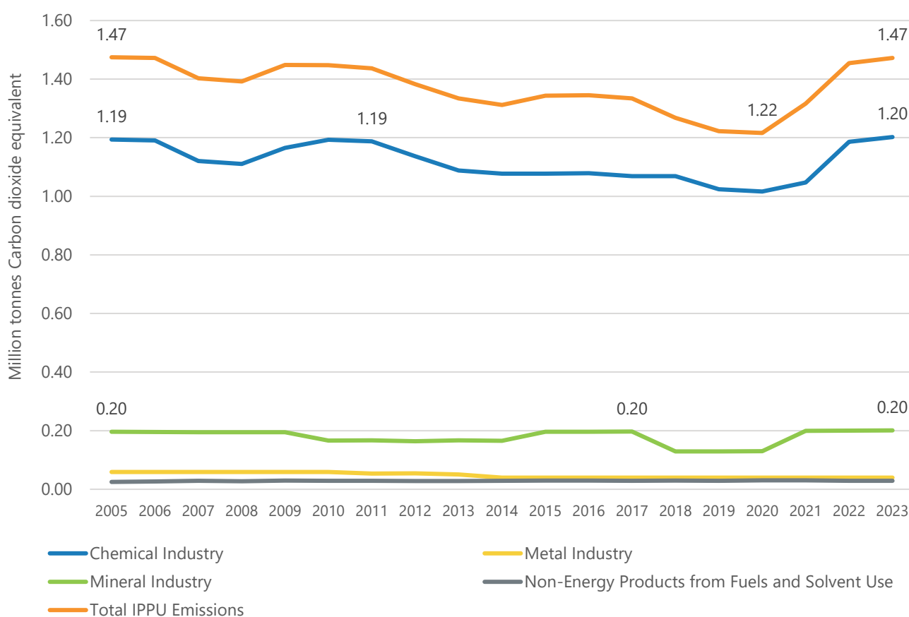
Figure-ER-13: Long-term Emissions Industrial Processes and Product Use (IPPU). The emissions trend is led by the Chemical Industry.
