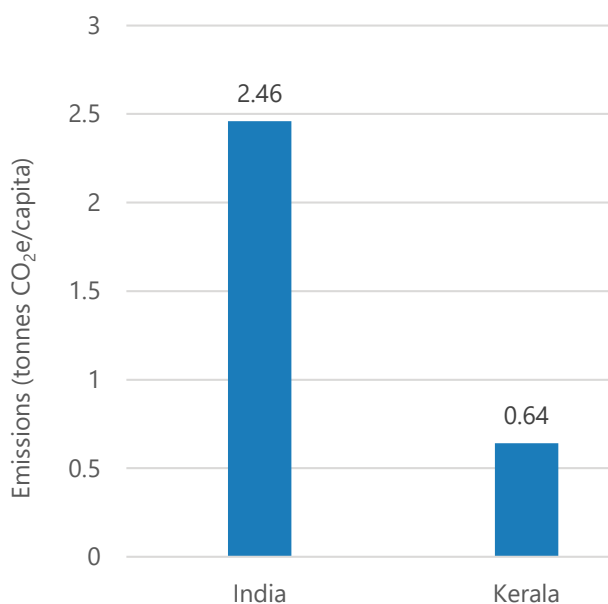
Figure-ER-2: Per Capita GHG Emissions -India and Kerala -2019- Based on Projected Population in the State for the year 2019 as per Census of India. India's per capita emissions for 2019, as per the latest estimates available with India's Long-term Low-Carbon Development Strategy submission to UNFCCC.
