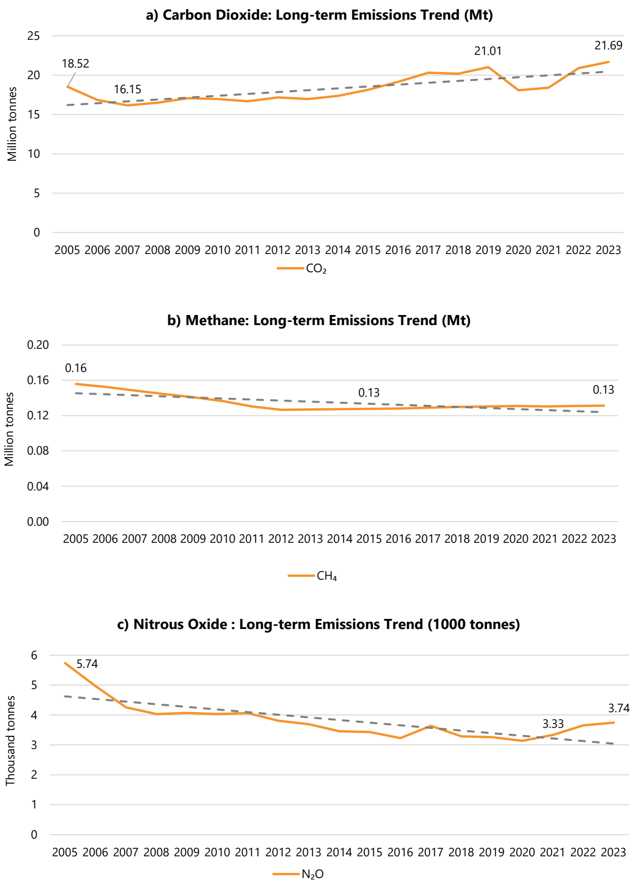
Figure-ER-7: Long-term emissions trend of various Greenhouse Gases. Panel (a) shows the Long-term emission trend of Carbon dioxide which shows an increasing trend, panel (b) shows the Long-term emission trend of Methane in (Million tonnes) and panel (c) shows the Long-term emission trend of Nitrous Oxide. Both methane and Nitrous Oxide show a declining trend in emissions. The dotted lines show the linear trend.
