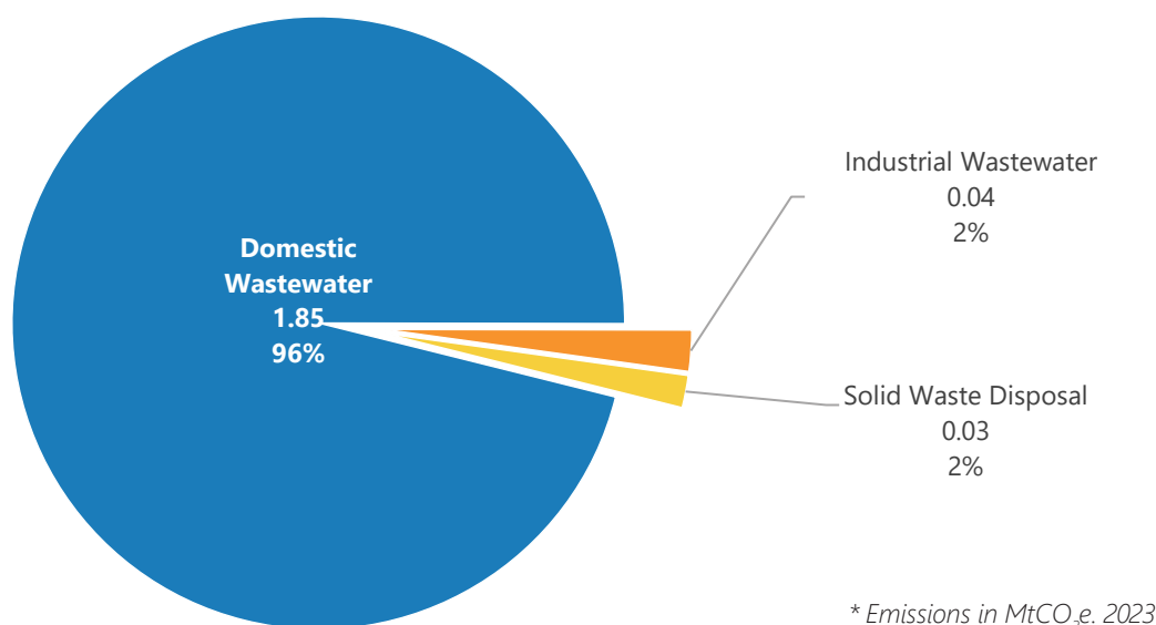
Figure-ER-21: Category-based Emissions and Percentage Shares in Total Waste Sector Emissions.
