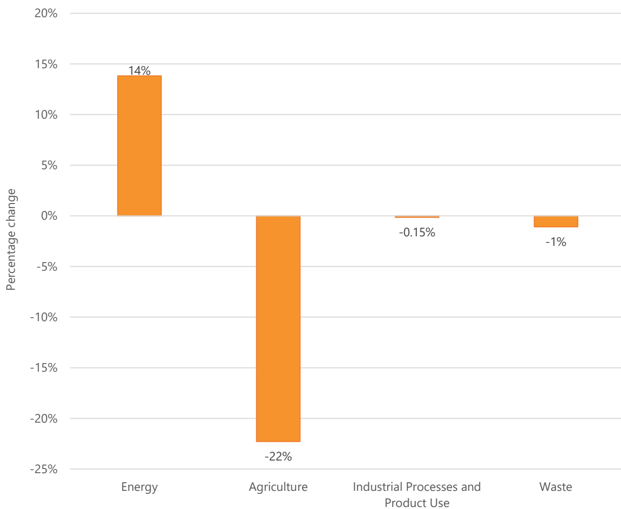
Figure ER-6: Changes in sector-based emissions in 2023 compared to 2005 baseline
