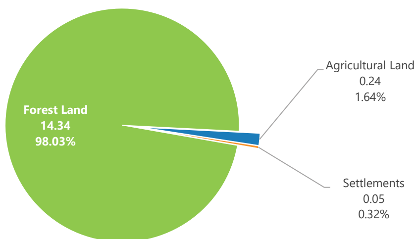
Figure-ER-19: Category-based Removals and their Percentage Shares (2023). Emissions from the LULUCF sector are proportionately very less in the case of Kerala. (~0.10% of total CO 2 sequestered)
