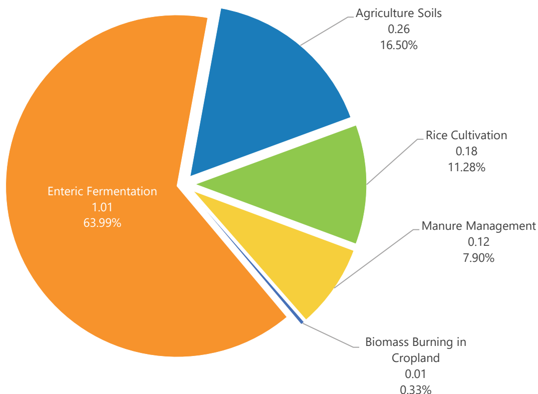
Figure-ER-17: Recent- Category-based Emissions in Agriculture and Percentage Share
