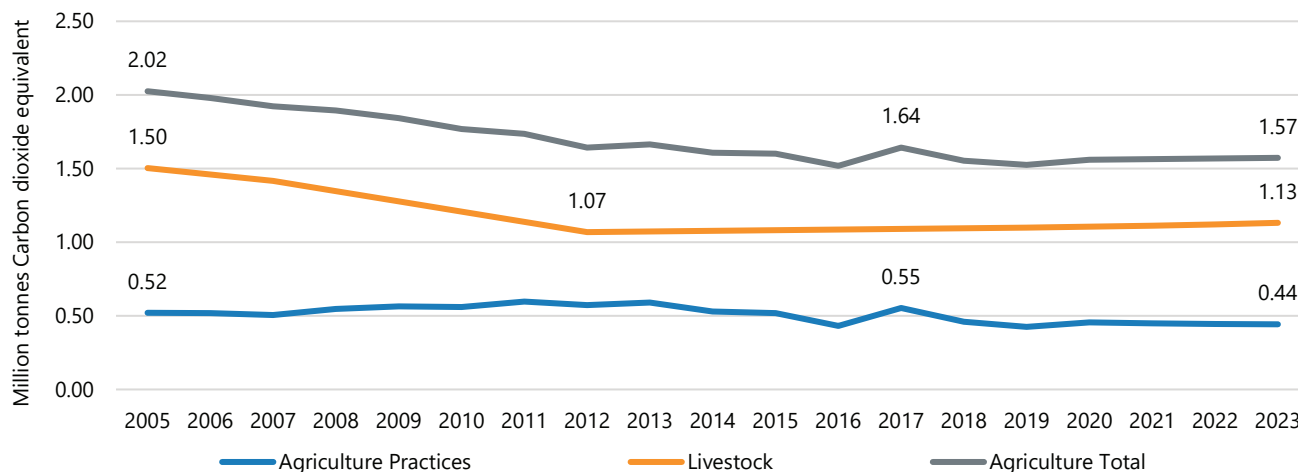
Figure-ER-15: Long-term emissions from the Agriculture Sector Agriculture total is the cumulation of emissions from agricultural practices and Livestock.
