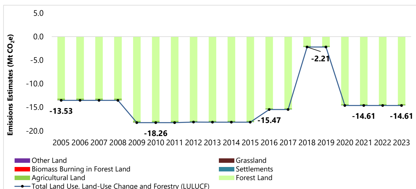
Figure 4: GHG Emissions Estimates of LULUCF Sector - Kerala (2005 to 2023)
