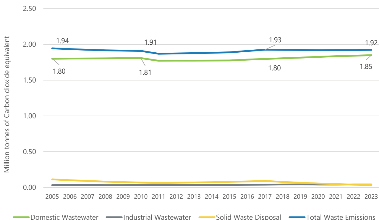
Figure-ER-20: Long-term GHG Emissions Estimates of Waste Sector
