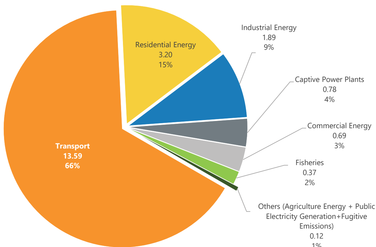
Figure ER-10: Category-based Emissions and Percentage Share in Total Energy sector Emissions (2023) - The figure shows the Category-based Emissions in MtCO 2 e and percentage share in total Energy sector Emissions in 2023. Transport and residential categories emit the maximum greenhouse gases in the State in 2023.
