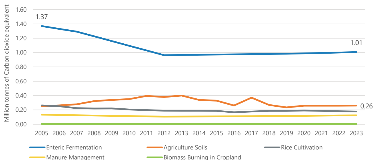
Figure-ER-16: Long-term Emissions- Various Categories in the Agriculture Sector
