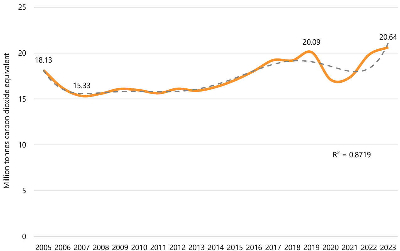
Figure-ER-8: Long-term emissions trend in the Energy sector.
