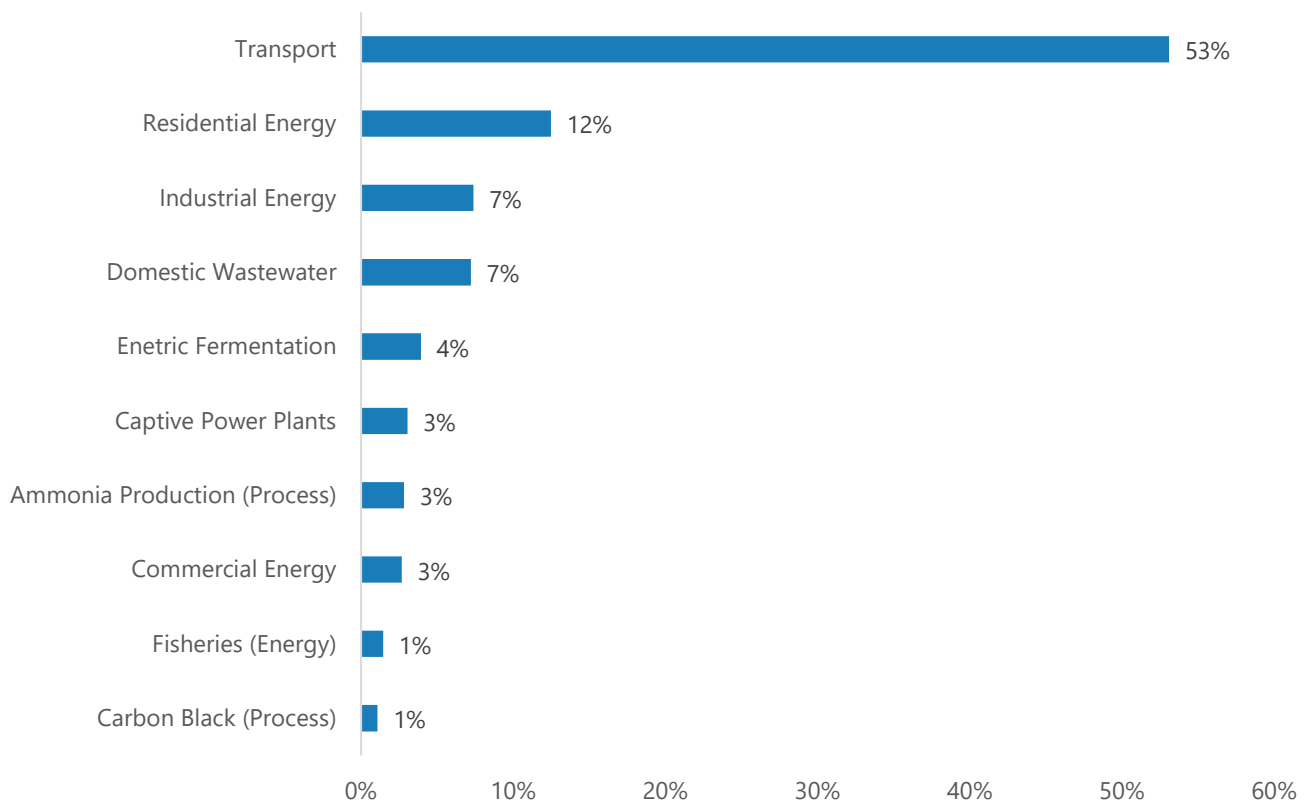
Figure-ER-23: Percentage share of Key Categories in overall Gross Emissions (2023)
