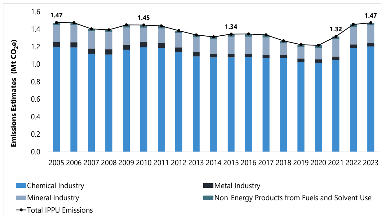
Figure 2: GHG Emissions Estimates of IPPU Sector – Kerala (2005 to 2023)
