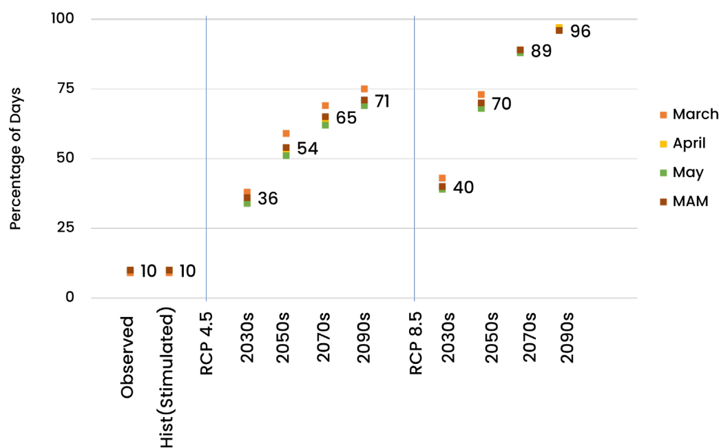
Figure 3.6: Observed, simulated, and projected percentage of warm days in Virudhunagar
