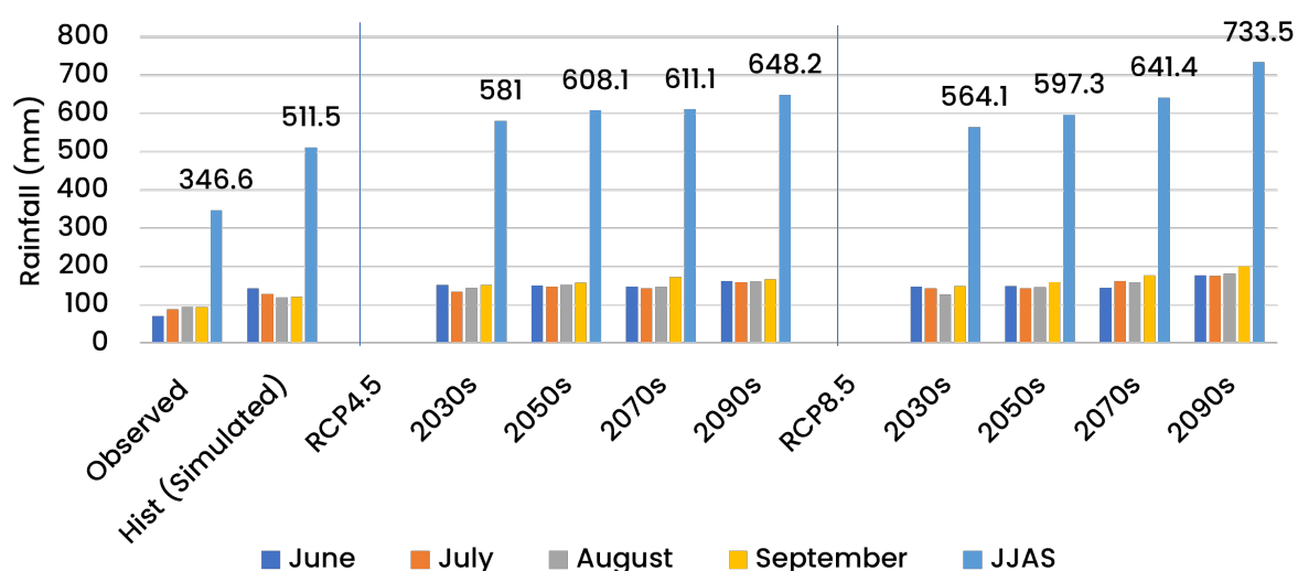
Figure 3.14: Observed (1986–2005), simulated (1986–2005) and projected mean monthly and southwest monsoon rainfall (mm) for Virudhunagar
