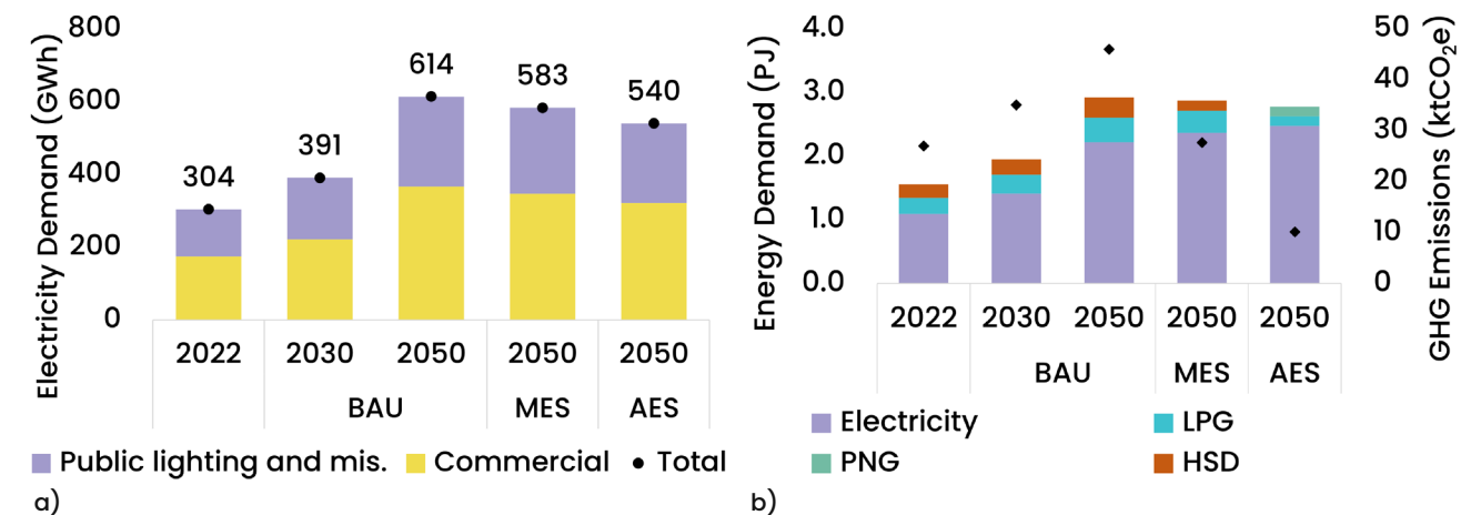
Figure 5.2 (a): Electricity demand in commercial building, (b) Energy and emissions in commercial buildings and public services in Virudhunagar
